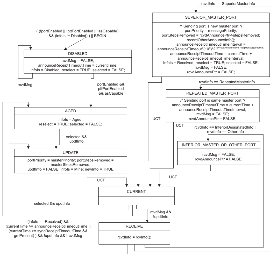
Figure 10-13—PortAnnounceInformation state machine
