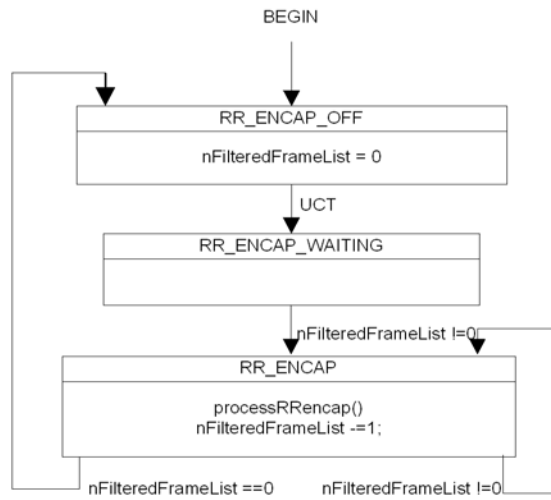
Figure 29-8—RR Encapsulation state machine
