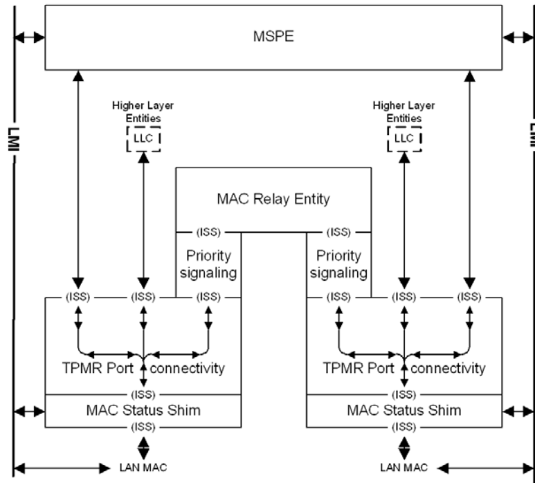
Figure 23-3—MSSs and the MSPE
