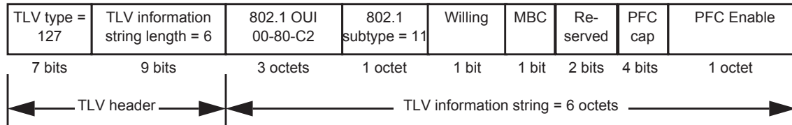
Figure D-11—Priority-based Flow Control Configuration TLV format
