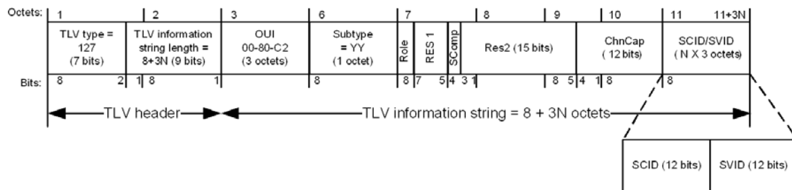
Figure D-14—CDCP TLV structure
