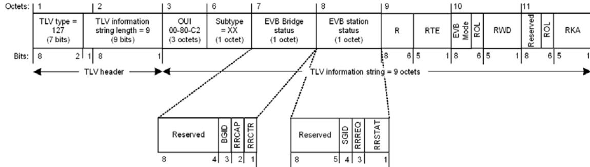
Figure D-13—EVB TLV format
