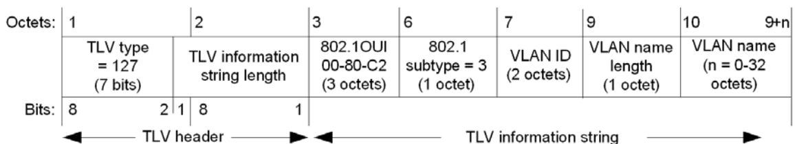
Figure D-3—VLAN Name TLV format
