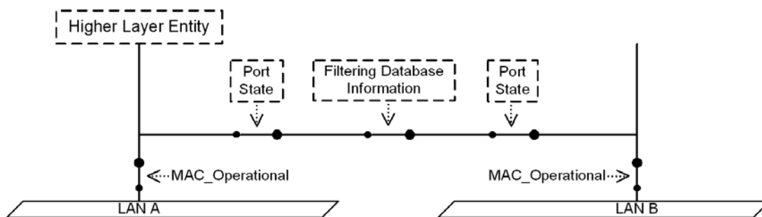
Figure 8-15—Single point of attachment—relay permitted
