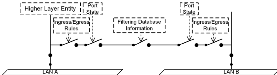
Figure 8-19—Ingress/egress control information in the forwarding path
