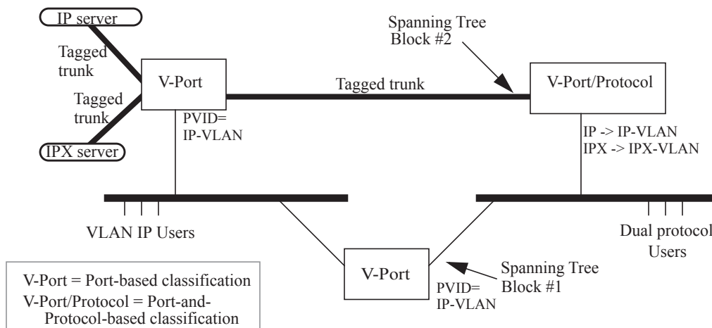
Figure H-4—Interoperability between Port-based and Port-and-Protocol-based classification
