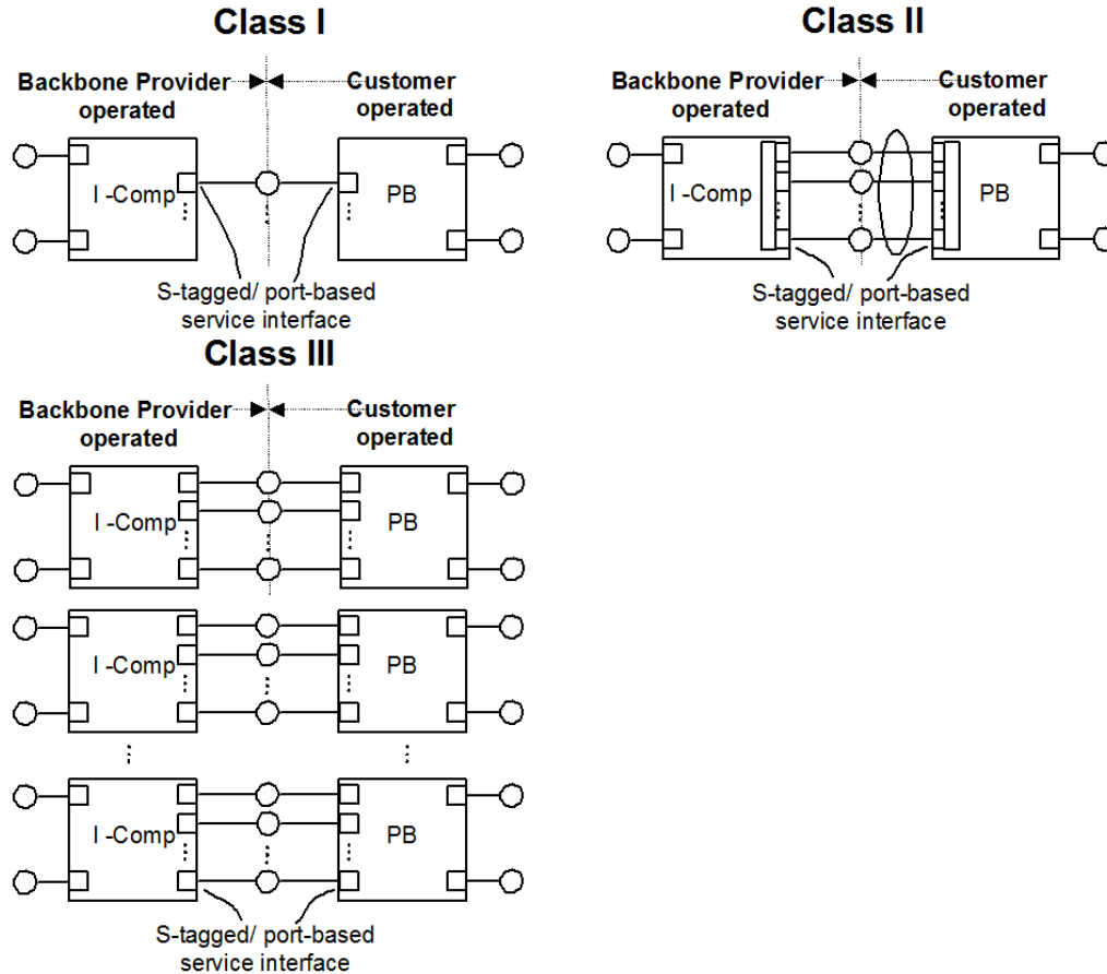
Figure 25-11—S-tagged and Port-based service interface access classifications
