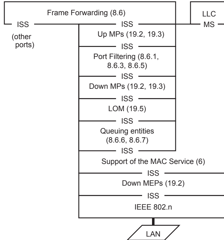
Figure 22-7—MP placement in a non-VLAN aware Bridge Port
