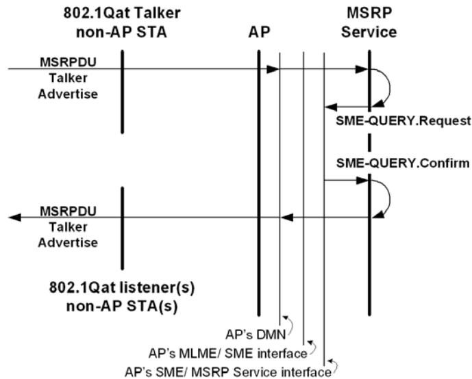
Figure C-10—MSRP/IEEE 802.11 query flows
