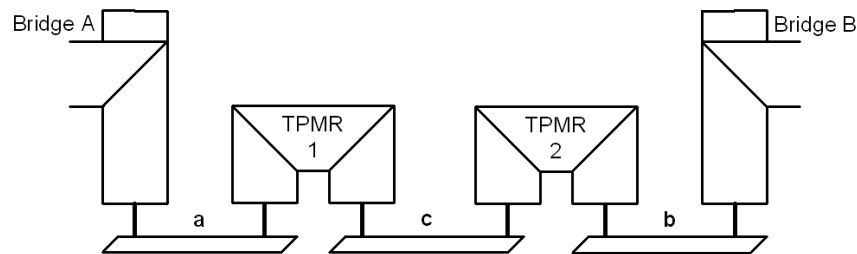
Figure 23-2—TPMP chain connecting Bridge Ports
