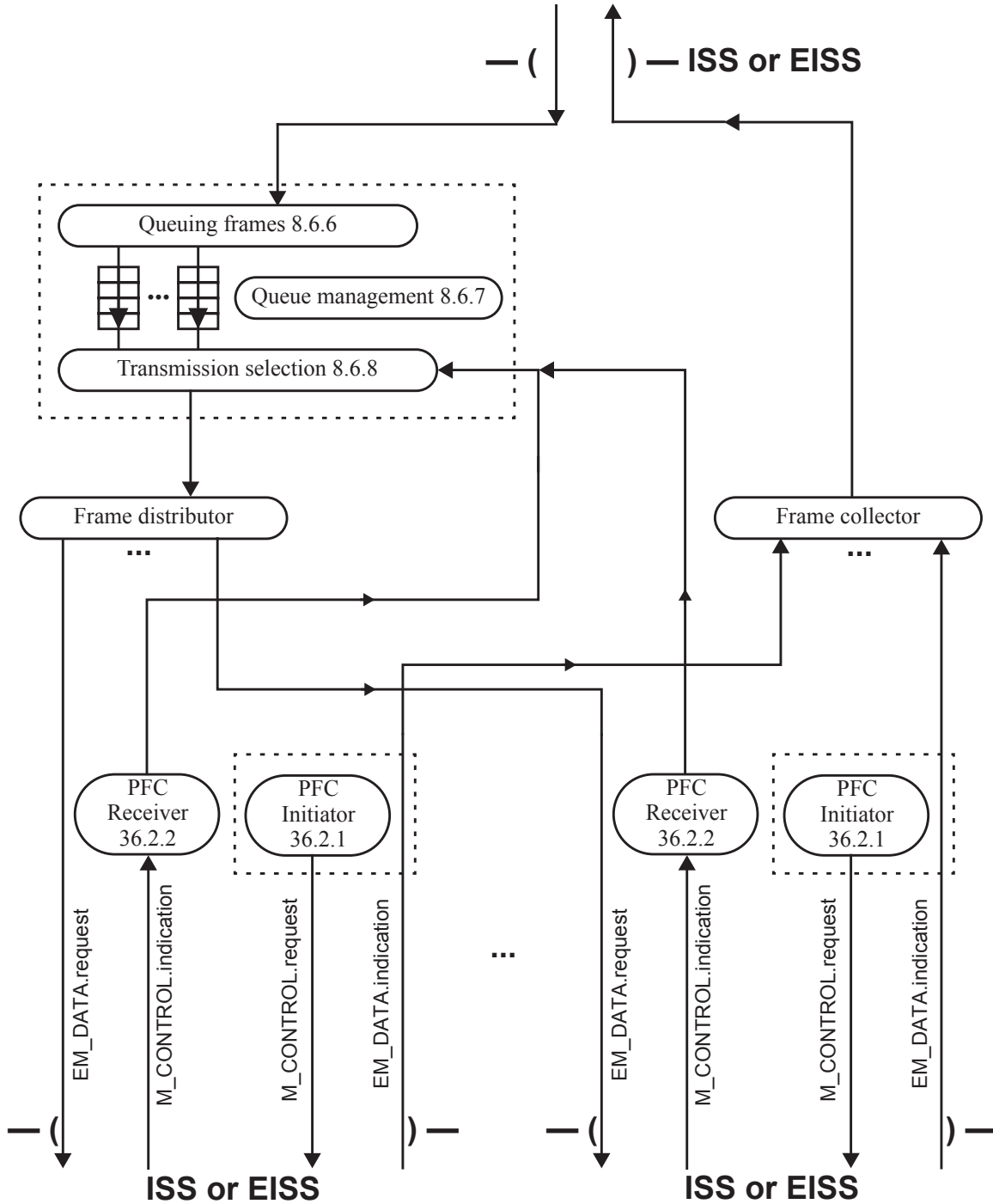
Figure 36-4—PFC aware system queue functions with Link Aggregation
