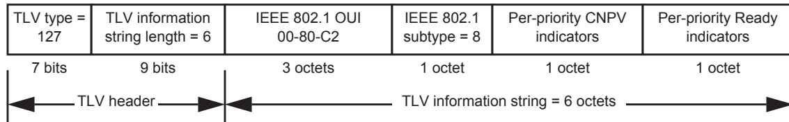
Figure D-8—Congestion Notification TLV format
