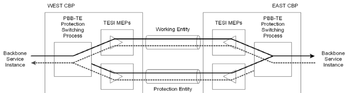
Figure 26-11—Protection switching architecture
