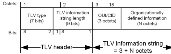
Figure 41-7—Organizationaly defined TLV
