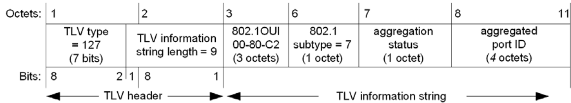
Figure D-7—Link Aggregation TLV format
