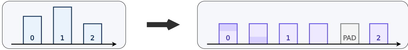
Figure 4: Example of segment downloads (left) replaced by cycles (right). Cycles can be full segment downloads (segment 2), partial segment downloads (1 and 0, where overlap between two cycles is indicated with shading), or padding.
