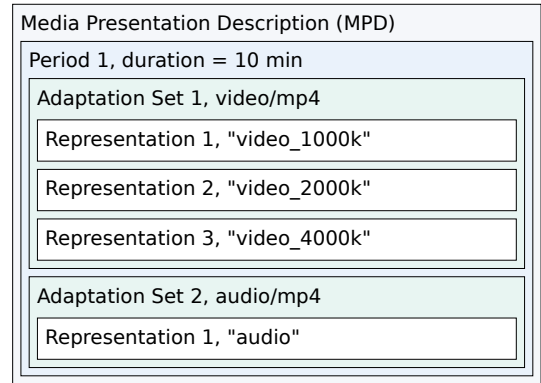
Figure 2: Manifest structure in DASH streaming.
