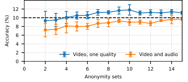
Figure 10: Accuracy (%), \mu \pm \sigma of vRF when training and testing on videos in different anonymity sets, with k = 10 .
