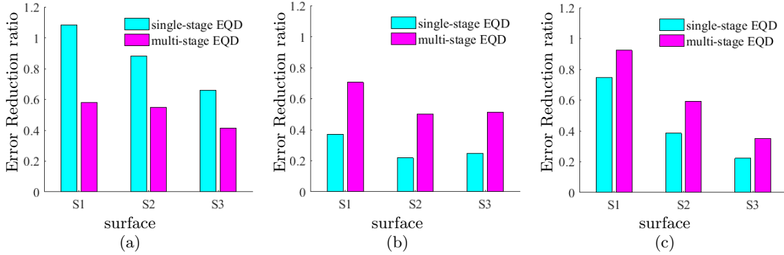
Figure 7: ER ratios for 2D systems: (a) S-shaped, (b) Load-response time, and (c) Bell-shaped.
