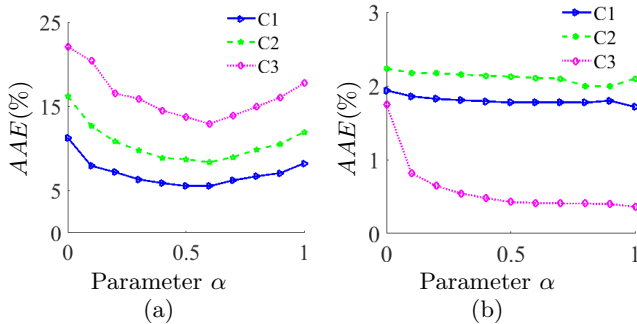
Figure 9: Effect of \alpha on AAE for 2D systems: (a) Load-response time, and (b) Bell-shaped.
