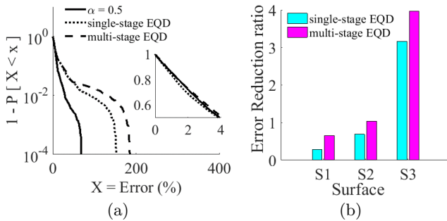
Figure 13: (a) cdf of errors and (b) ER ratios for 0.1 < R < 0.4 .
