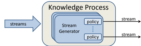
Figure 1. A prototypical knowledge process.
