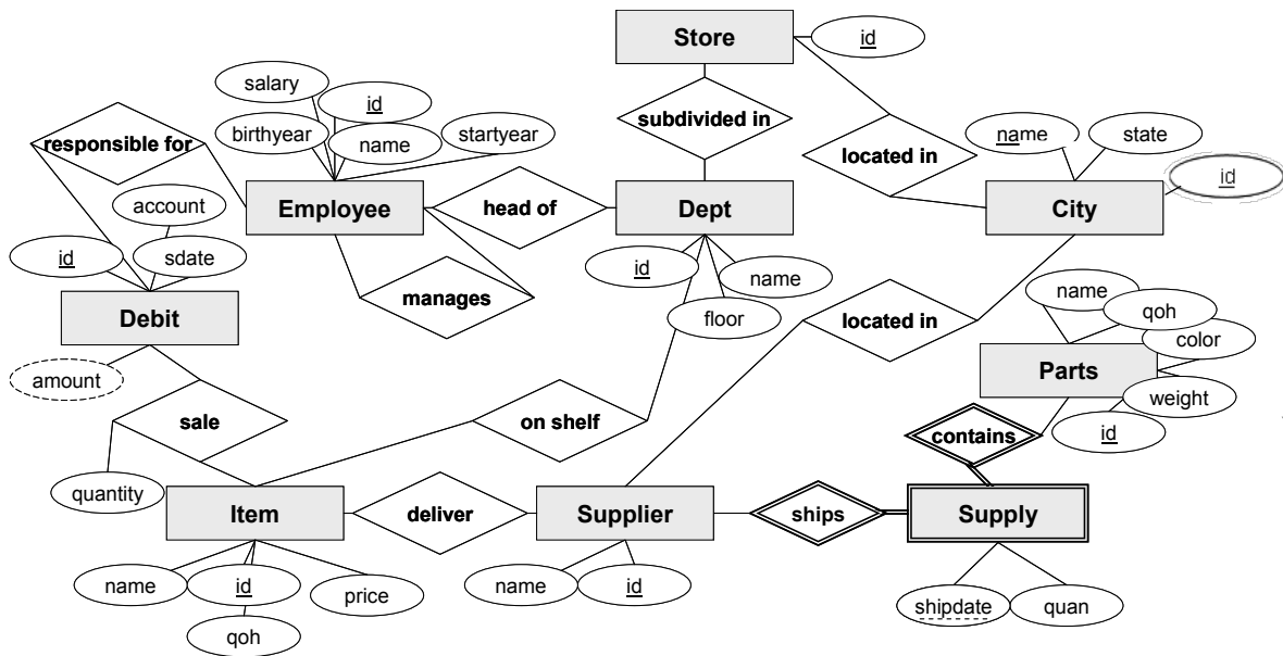
The Jonson Brothers' ER-Diagram (The cardinalities are left to fill in as an exercise)
