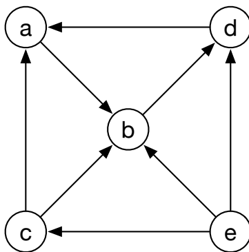
Figure 2: G_4
