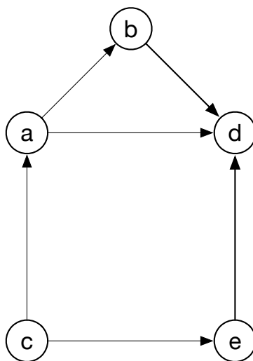
Figure 1: G_3
