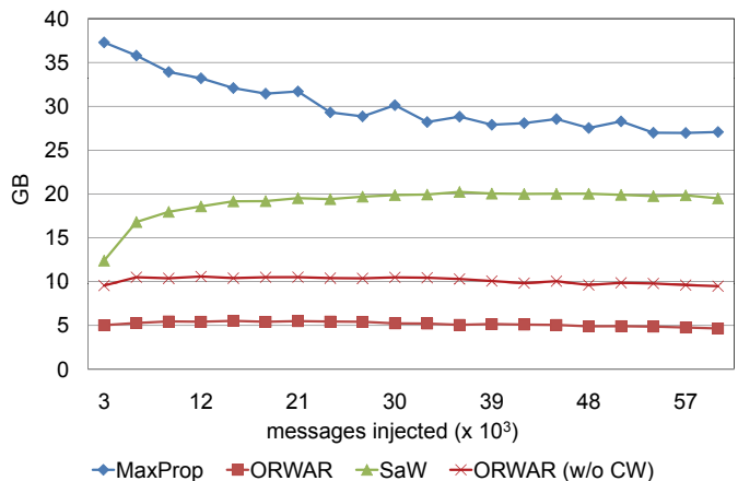
Figure 7: Partial transmission total size versus load
