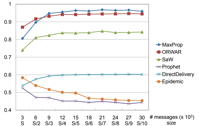
Figure 5: Delivery rate versus message size
