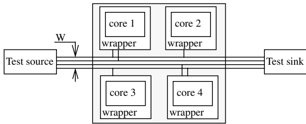
Figure 5. SoC example.
