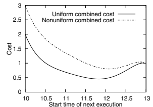
Figure 5. Combined control and CPU costs. Two different combinations of the control task and are in general conflicting objectives.
