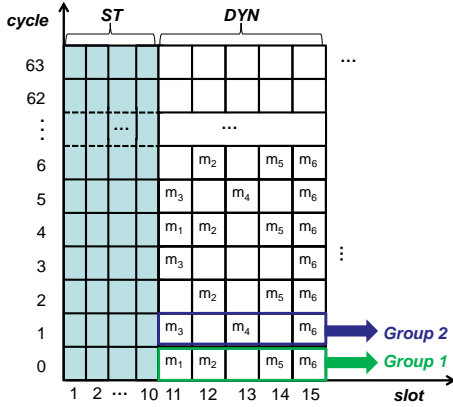
Fig. 6. Groups of the DYN segment messages.
