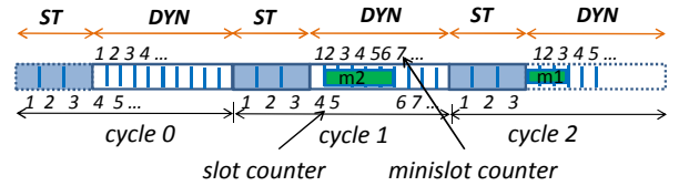
Fig. 2. Transmission over the DYN segment.
