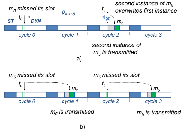
Fig. 4. Scenarios for message transmission with different repetition rates a) R_5 = 2 , b) R_5 = 1 .
