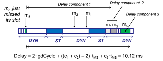
Fig. 5. The worst case delay scenario for m_5 .
