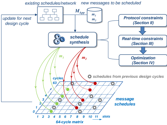
Fig. 1. Overview of our incremental schedule synthesis engine.
