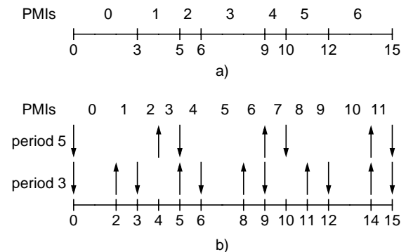
Figure 5. Priority monotonicity intervals
