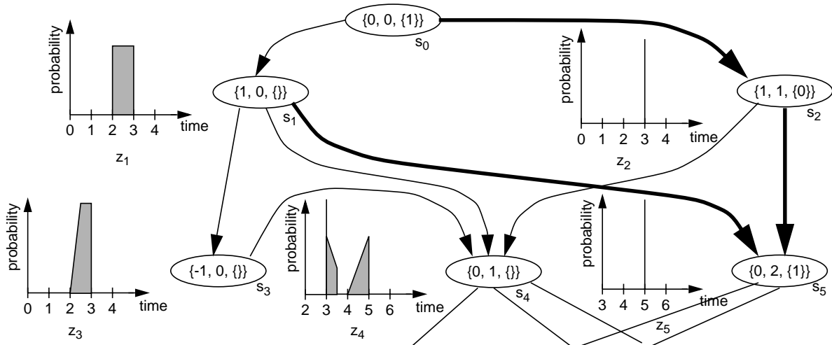
Figure 7. Stochastic process example
