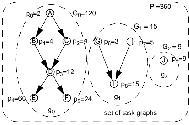
Figure 1. Set of task graphs
