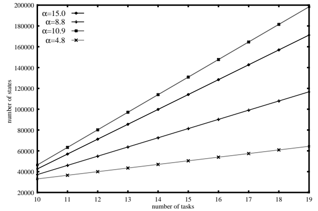
Figure 10. Experiment 1, stochastic process size
