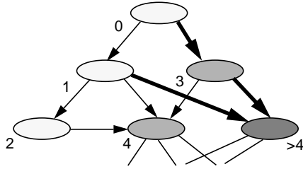
Figure 9. State selection order
