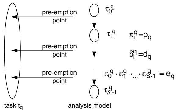
Figure 3. Introducing pre-emption points
