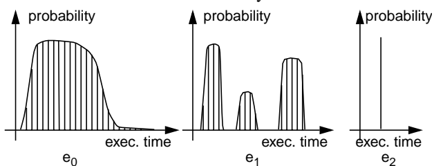
Figure 2. Exec. time probability density functions
