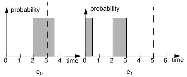
Figure 4. ETPDFs for tasks t_0 and t_1
