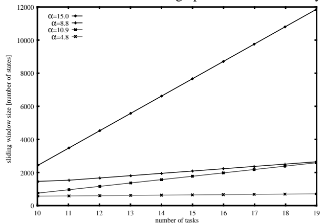
Figure 11. Experiment 1, sliding window size
