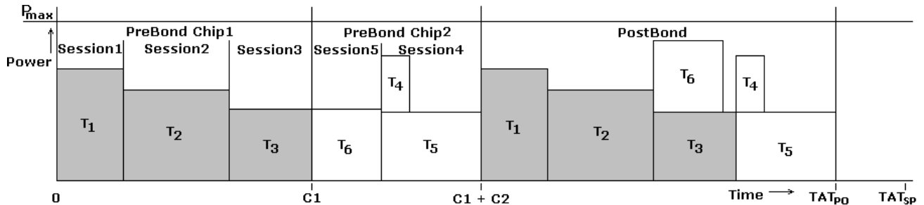
Figure 5: Partial Overlapping
