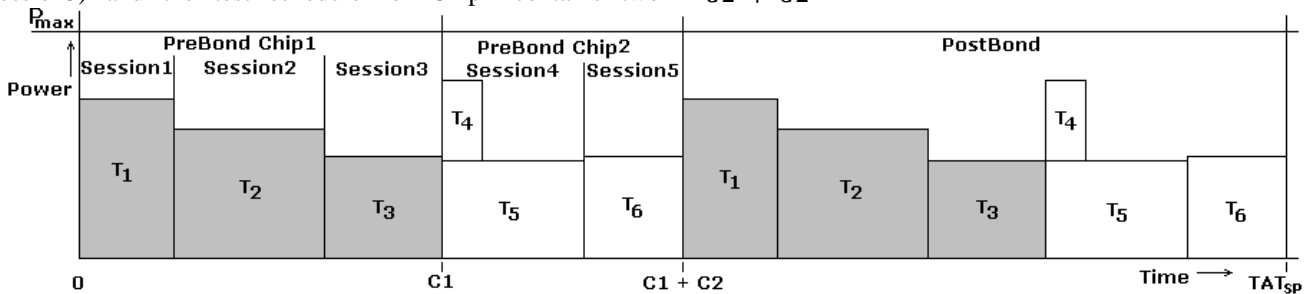
Figure 4: Serial Processing.
