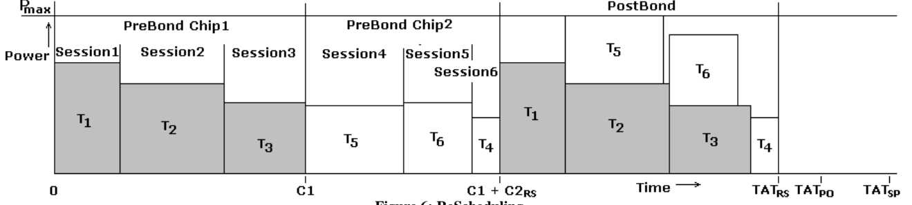
Figure 6: ReScheduling
