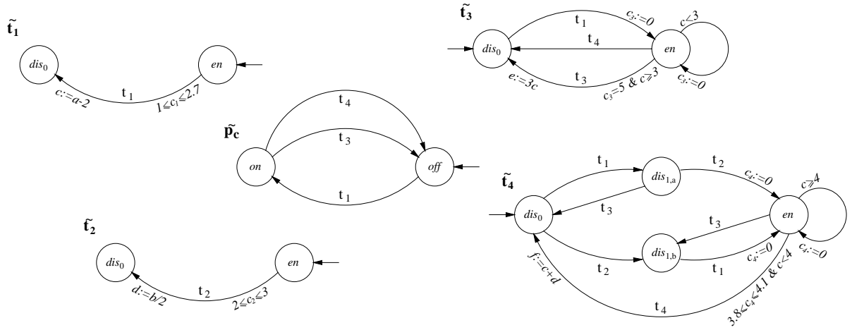
Figure 2. Equivalent hybrid automata
