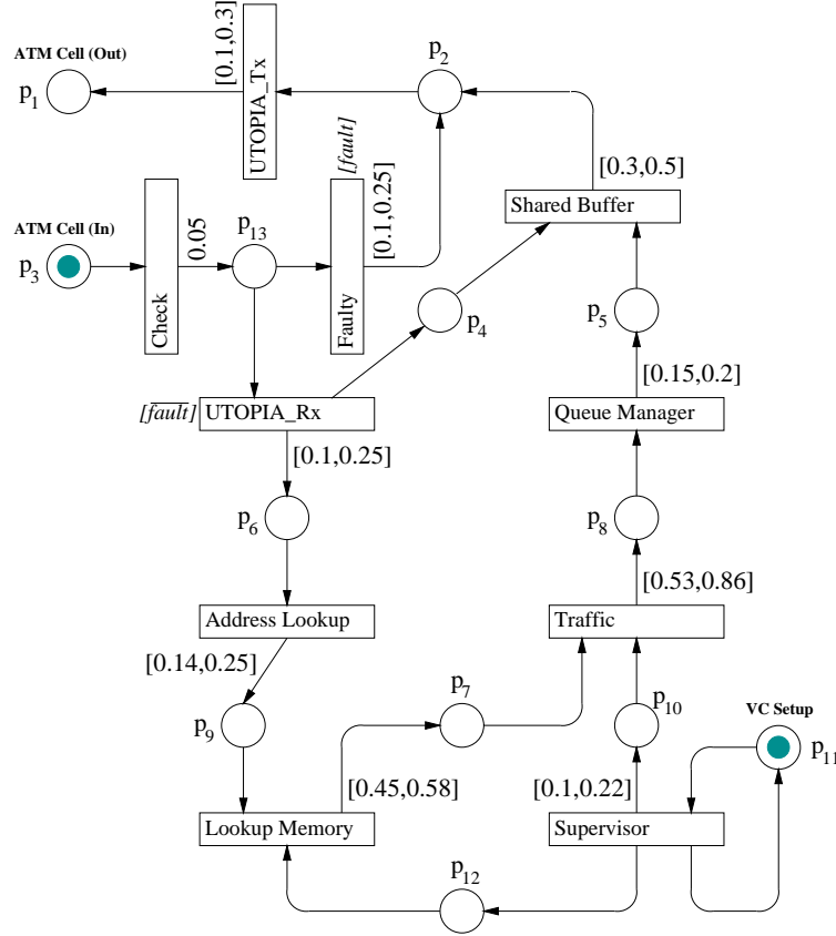
Figure 4. PRES+ model of an A-VPN server
