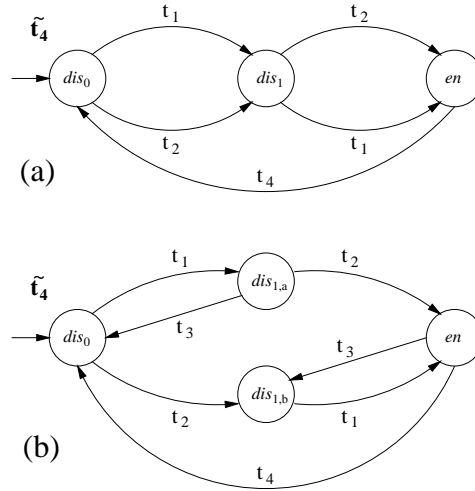
Figure 3. Illustration of Step 4
