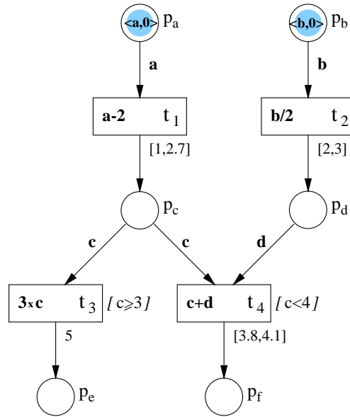
Figure 1. A PRES+ model
