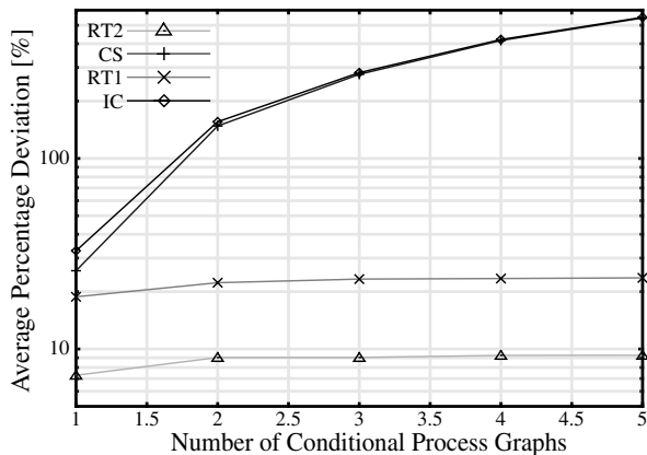
Figure 11. Avg. Deviations Based on the No. of CPGs
