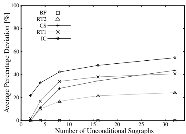
Figure 10. Deviations, No. of Unconditional Subgraphs
