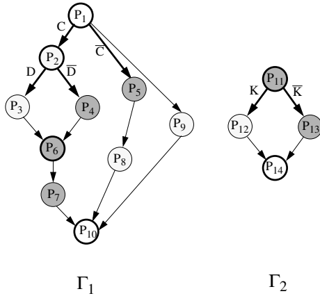
Figure 4. Example of two CPGs
