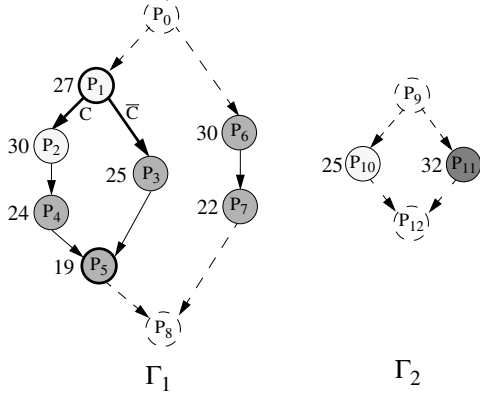
Figure 2. System with Control and Data Dependencies
