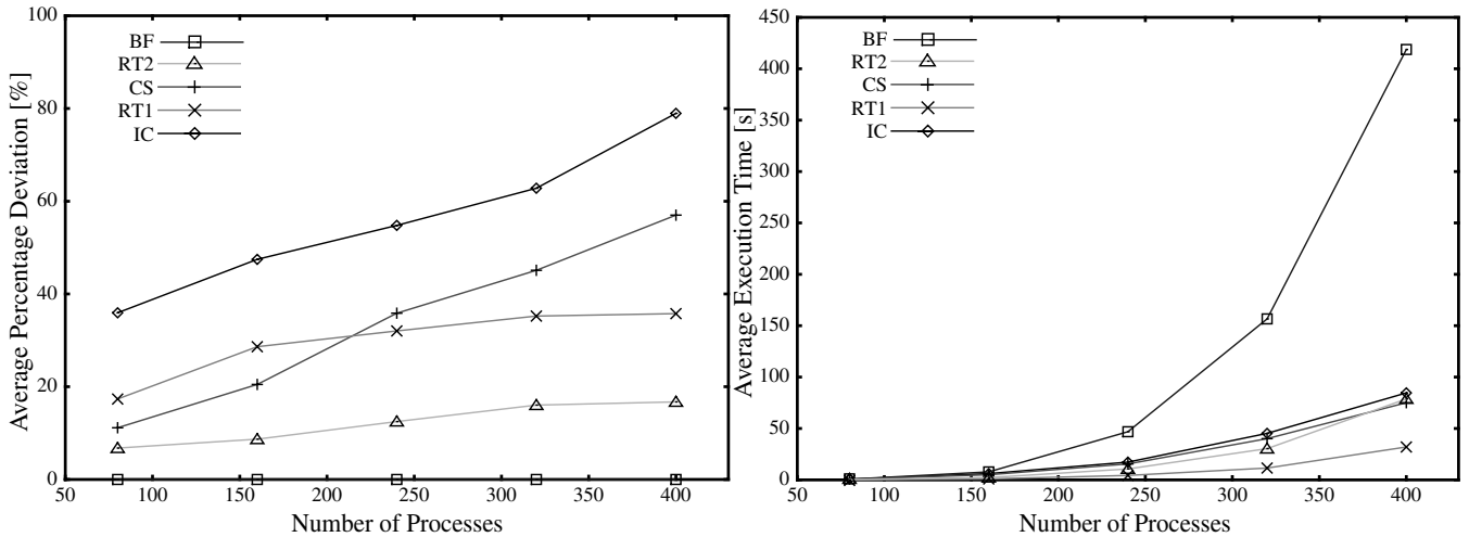
Figure 9. a) Average Percentage Deviation (left) and b) Average Execution Time (right) for each of the five analyses
