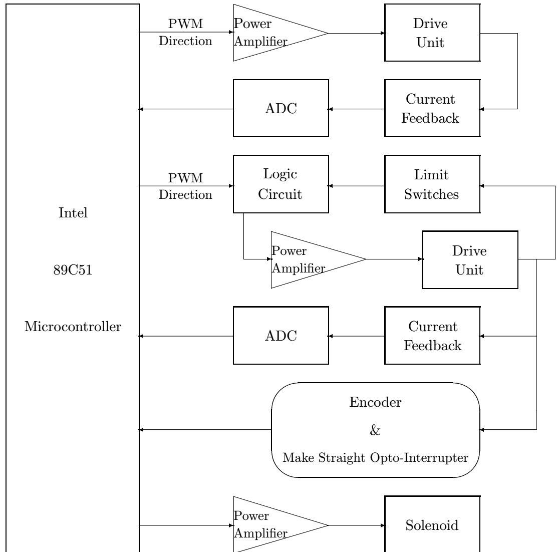
Figure 1: The Arvand control diagram. Each robot has two of these circuits, one for each side of the robot.
