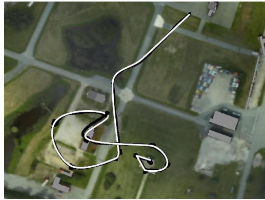
Fig. 8. Autonomous survey mission to building1 and then building2 photographed from each side.
