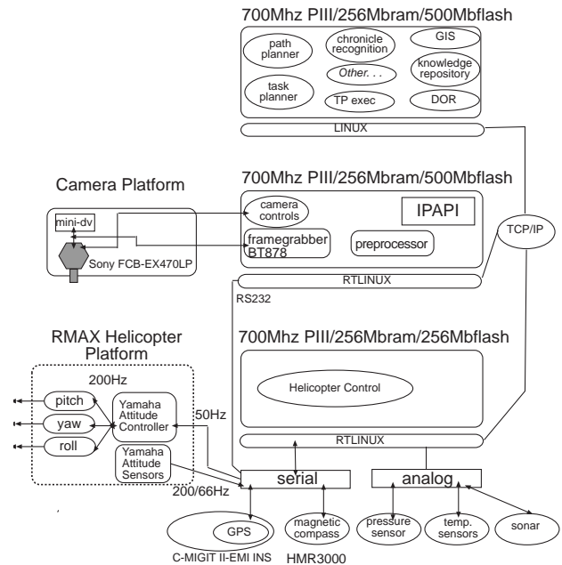
Fig. 3. On-Board Hardware Schematic
