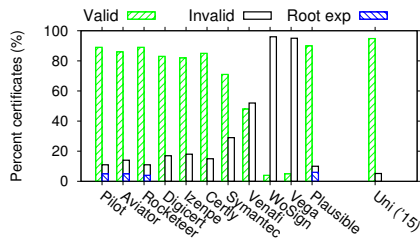
Fig. 3. Validation tests using the Mozilla root store.
