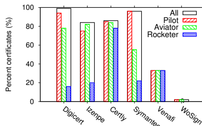
Fig. 4. Percent of entries in CA operated logs seen in at least one Google log.
