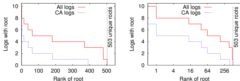
Fig. 1. Number of logs accepting each root for submitted entries.
