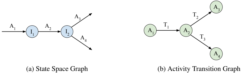
Figure 3. A denotes an activity in both the State Space Graph and the Activity Transition Graph, I denotes an intersection point in the state space, T denotes a transition in the Activity Transition Graph. All transitions between A_2 , A_3 and A_4 can be seen as contained within the intersection point I_2 .
