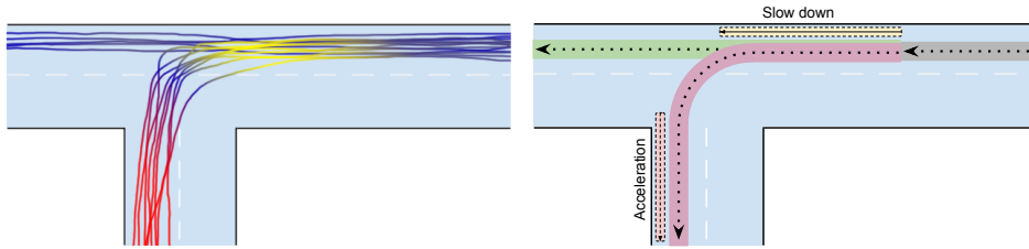
Figure 1. An illustrative example of the expected input and output of the proposed framework. The left figure shows observed trajectories. Blue is constant velocity, yellow is negative acceleration, and red is positive acceleration. The right figure shows a conceptual illustration of what we want to learn.
