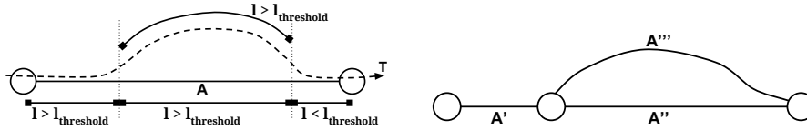
Figure 5. Illustrative example of the create procedure , where the left figure is before and the right figure is after. The dotted lines indicate where the similarity of A and T is crossing the s_{threshold} .
