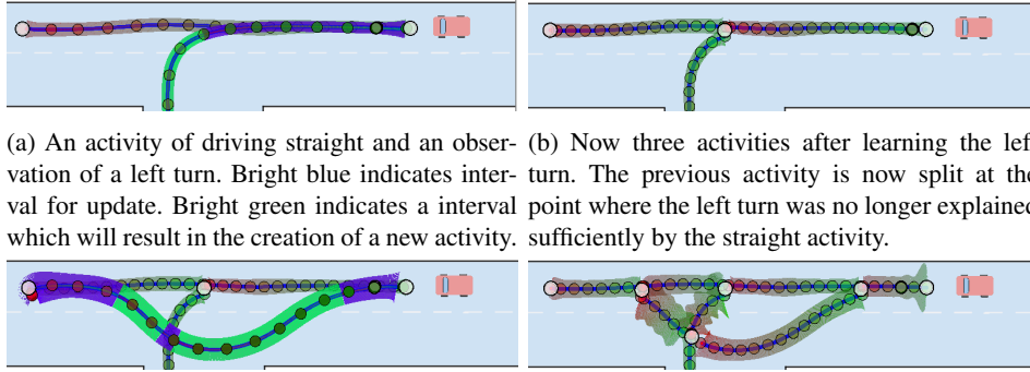
(c) An illegal overtake is observed. The rounded trajectory of the overtake is indicated to be created as two activities since it is too similar to the left turn when spatially crossing it. This do not happen if velocities are part of the state space. (d) After the overtake has been learned. The highly varying variance seen on the shorter activities is due to the parameters of the kernels not being updated properly.
