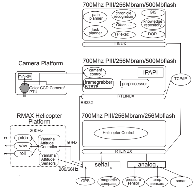
Figure 2: DARA Hardware Schematic
