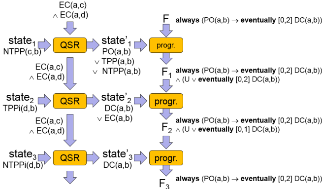
Figure 2. A qualitative spatio-temporal stream reasoning example.
