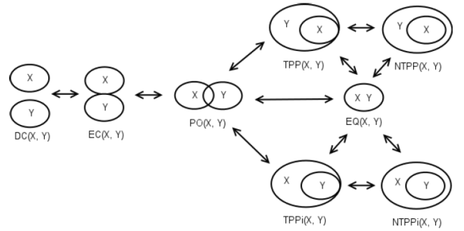
Figure 1. The RCC8 relations and their continuity network.
