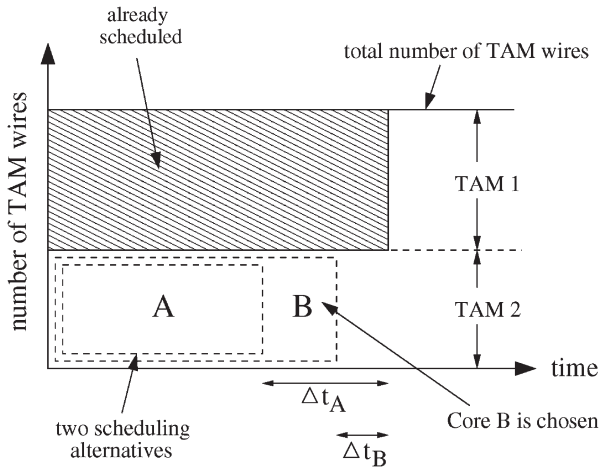
Fig. 5. Illustration of the best fit principle used in the test scheduling algorithm.
