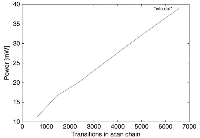
Fig. 6. Total transition count versus power dissipation for s5378.
