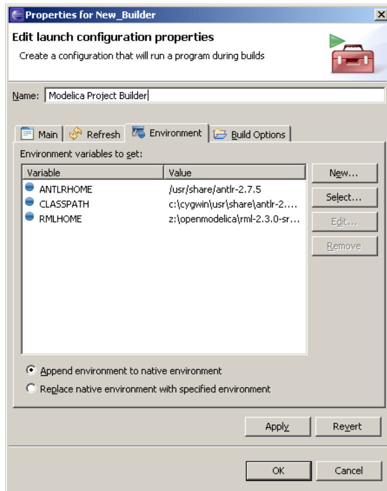
Figure 7: Environment properties
