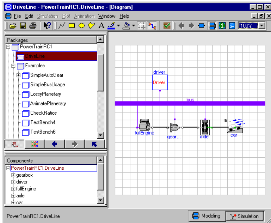
Figure 11: Dymola
