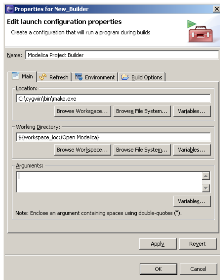
Figure 6: Properties for Modelica Project Builder
