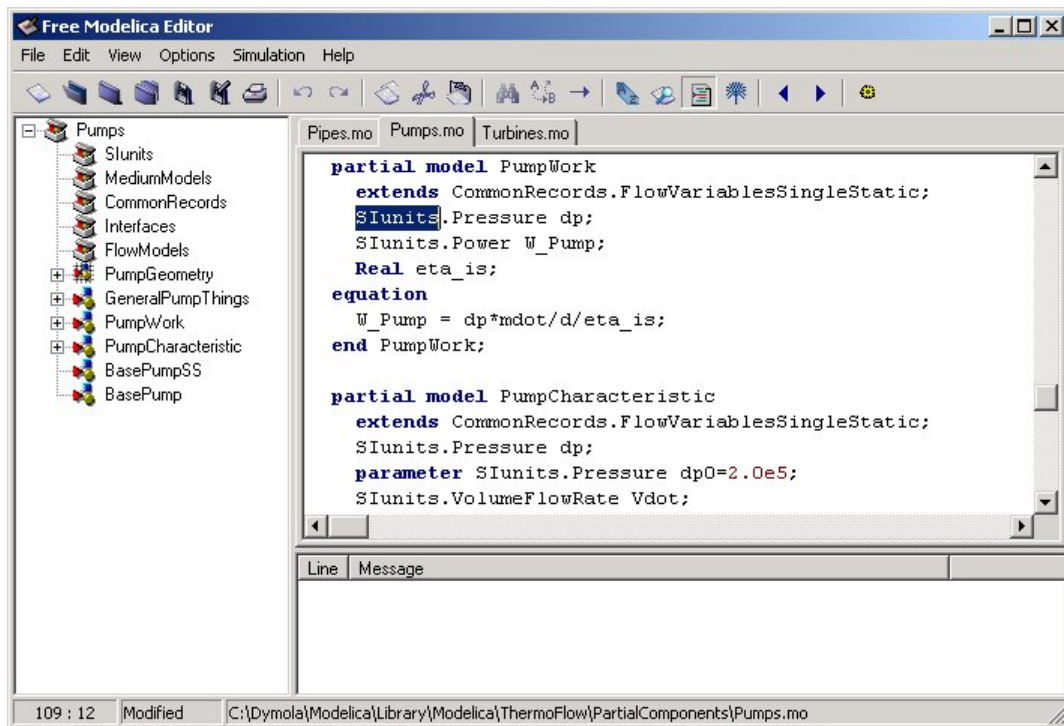
Figure 13: The Free Modelica Editor
