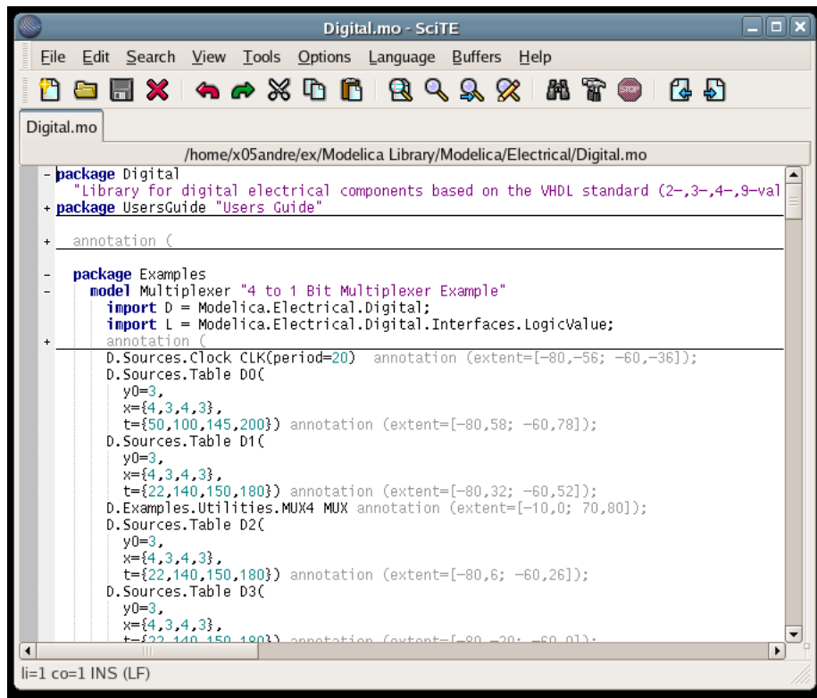
Figure 15: SciTE
