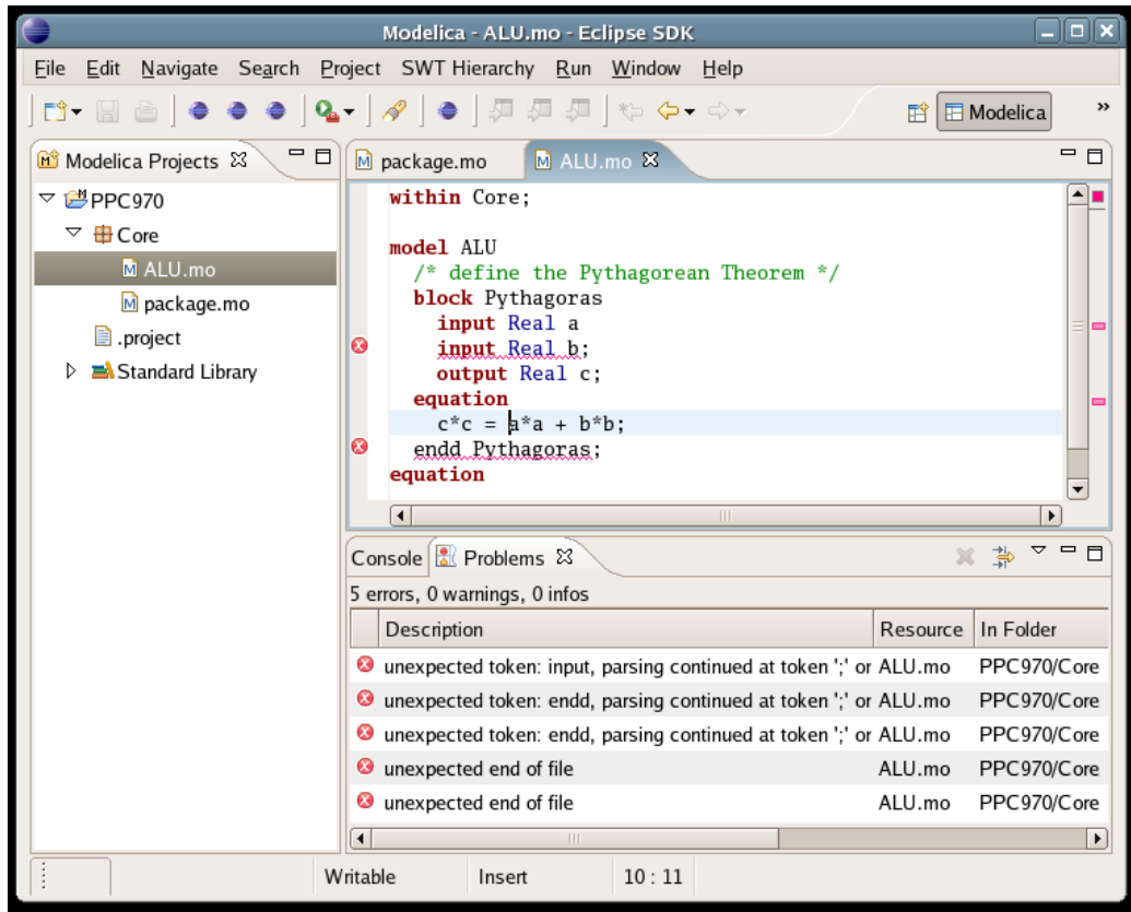
Figure 10: Modelica Perspective
