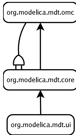
Figure 9: MDT Plugins Architecture
