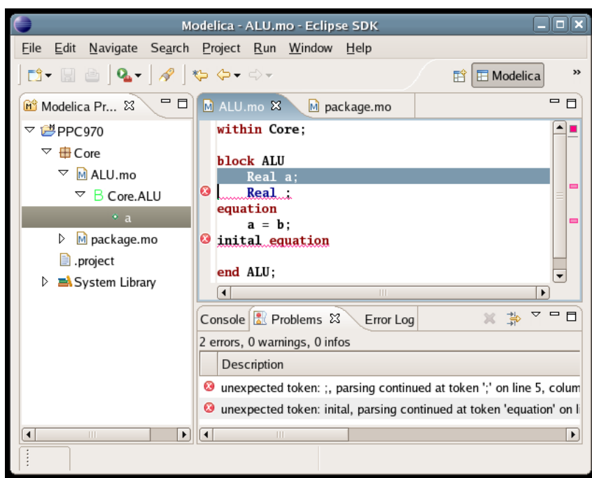
Figure 5: Syntax errors
