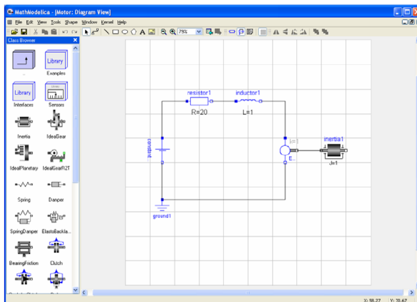
Figure 12: MathModelica
