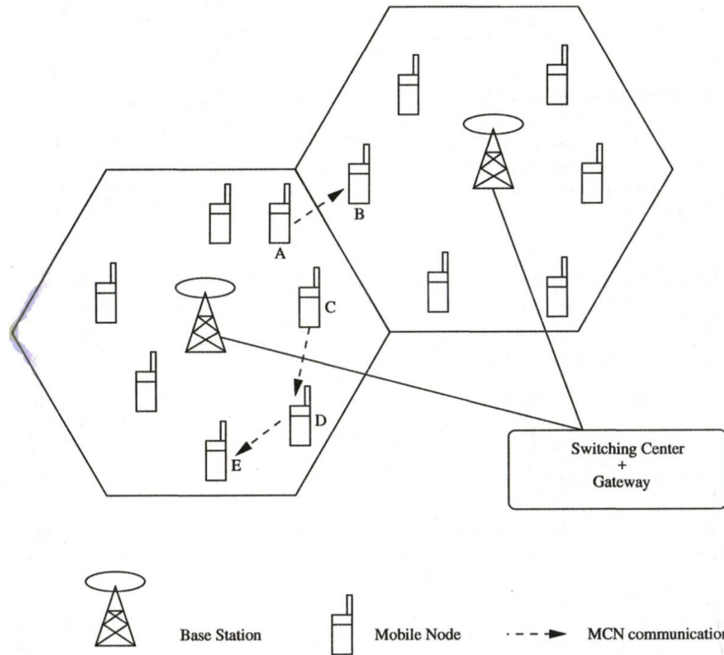
Figure 5.6. MCN architecture.
