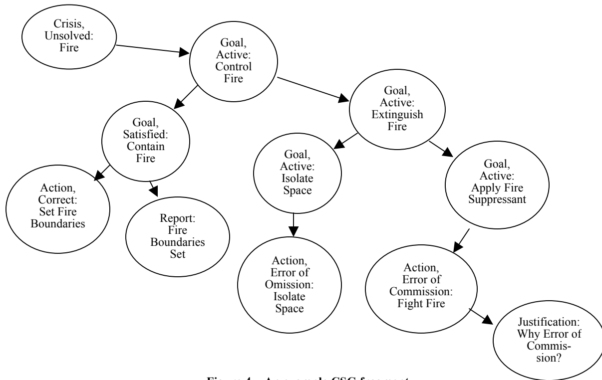
Figure 4 – An example CSG fragment.
