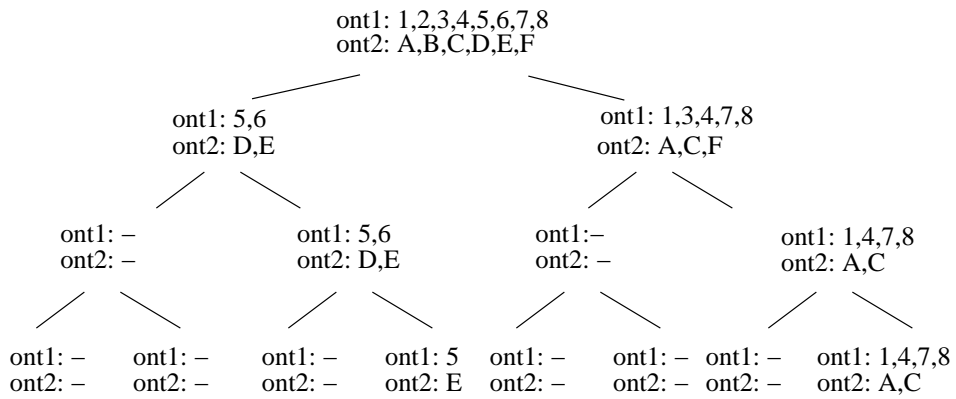
Figure 4: Binary tree after using (2,B), (3,F) and (6,D) – without pruning.
