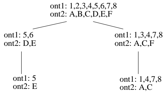
Figure 4: Binary tree after using (2,B), (3,F) and (6,D) – with pruning.
